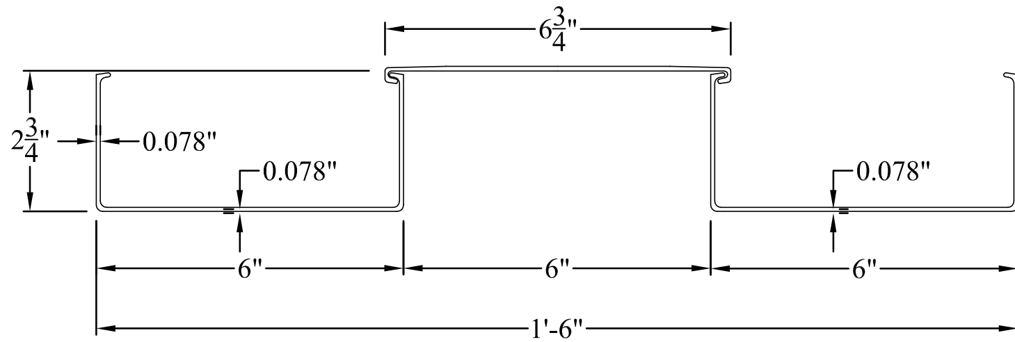
1 2-3/4" DECK ASSEMBLY
