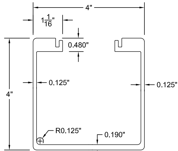
1 4" X 4" GUTTER BEAM
